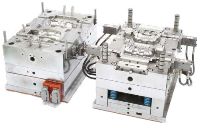
Car Head Restraint Mold
